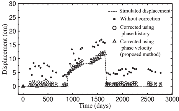
Fig. 6. Comparison of DEM error corrections in the time domain using phase velocity history and phase history. The DEM error is best estimated in the time domain from the phase velocity.
